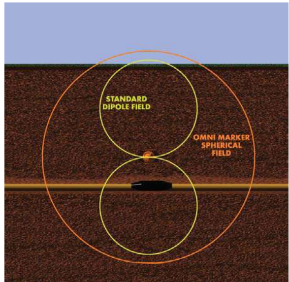
Omni Marker spherical field compared to the standard 3M Ball Marker dipole field.
